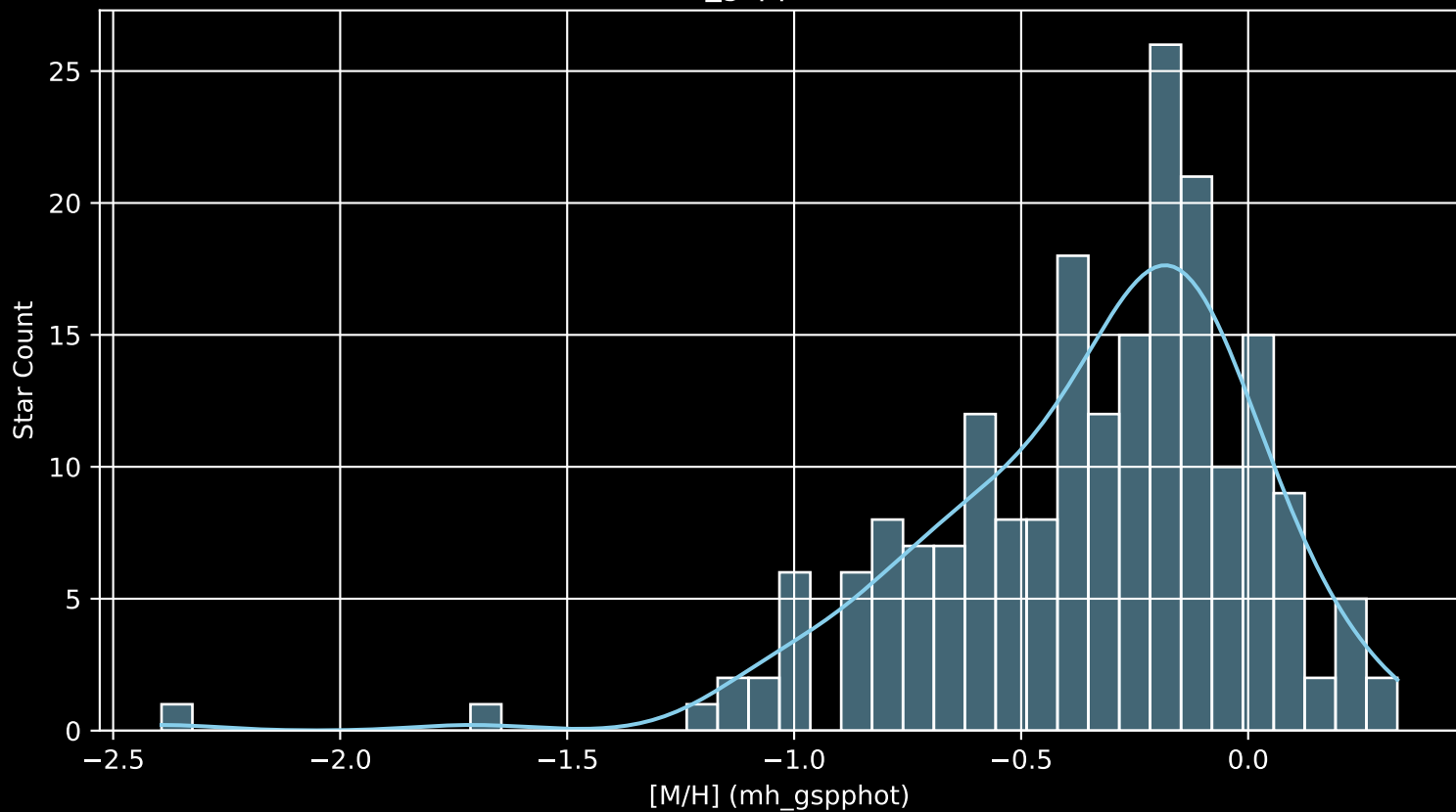
APOGEE DR17 Field: [180-30 [M/H] (mh_gspphot) (n= 204)
