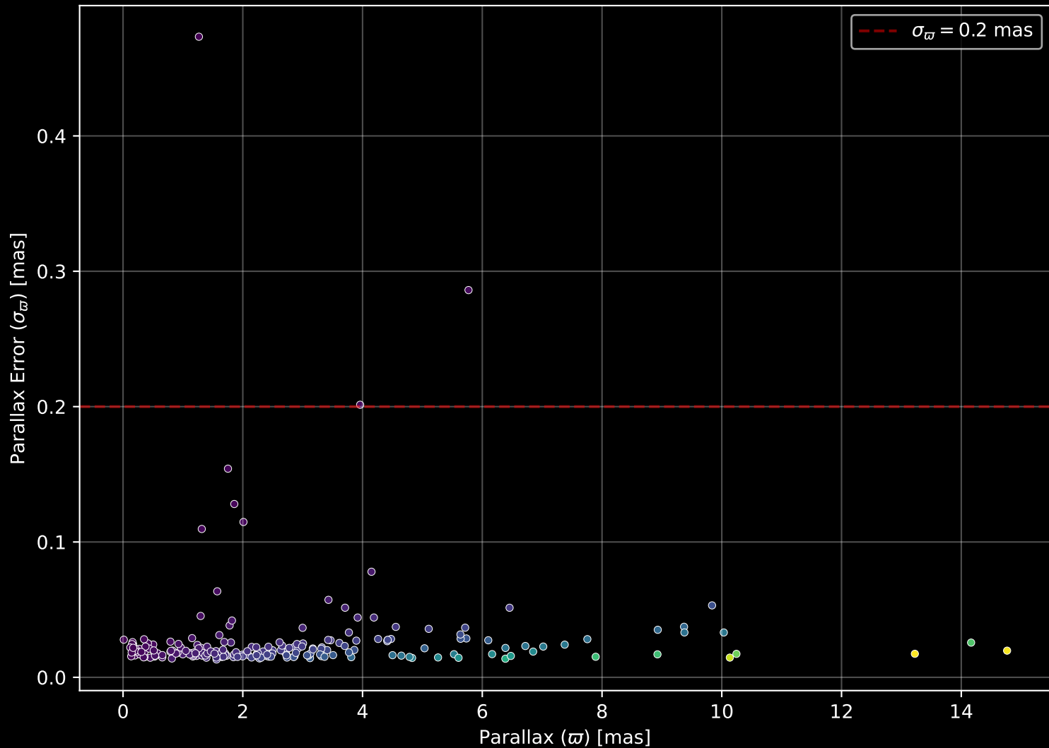
APOGEE DR17 Field: [180-30] Parallax Quality (n= 206)
