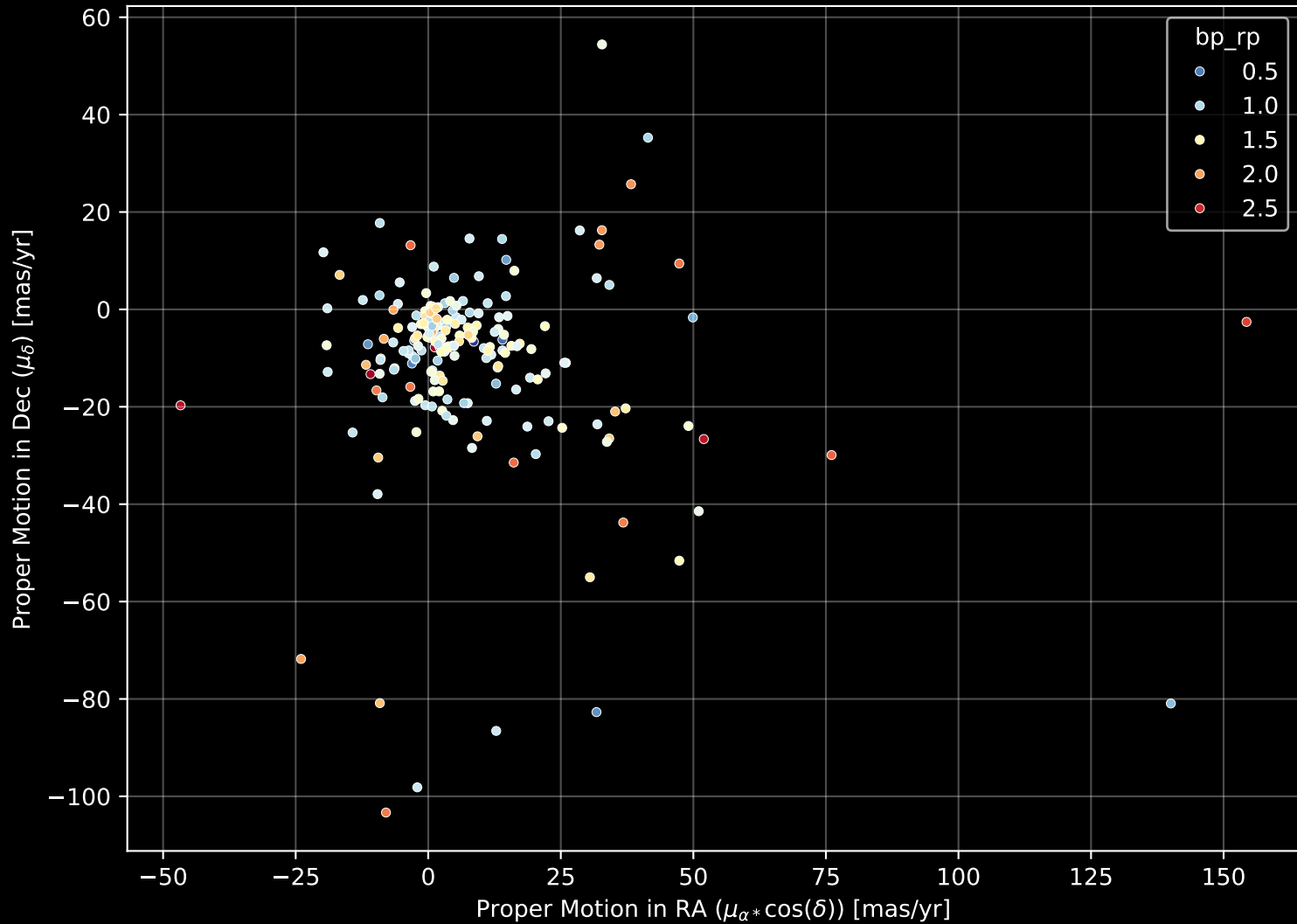
APOGEE DR17 Field: [180-30] Proper Motion Diagram (n= 206)
