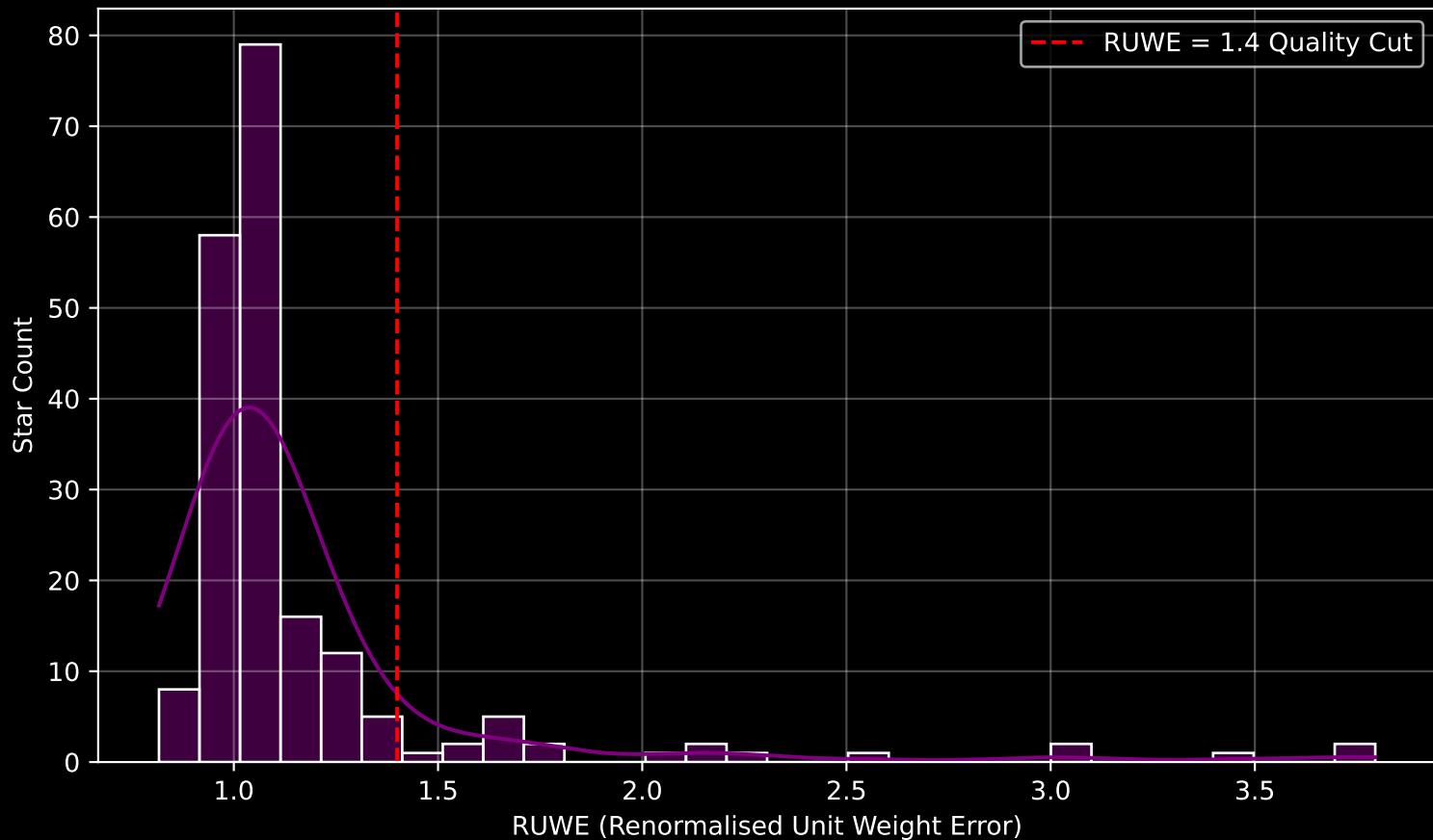
GAPOGEE DR17 Field [180-30] RUWE Distribution (n= 198)
