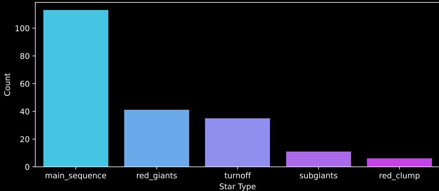
APOGEE DR17 Field: [180-30] Count plot of Star Type
